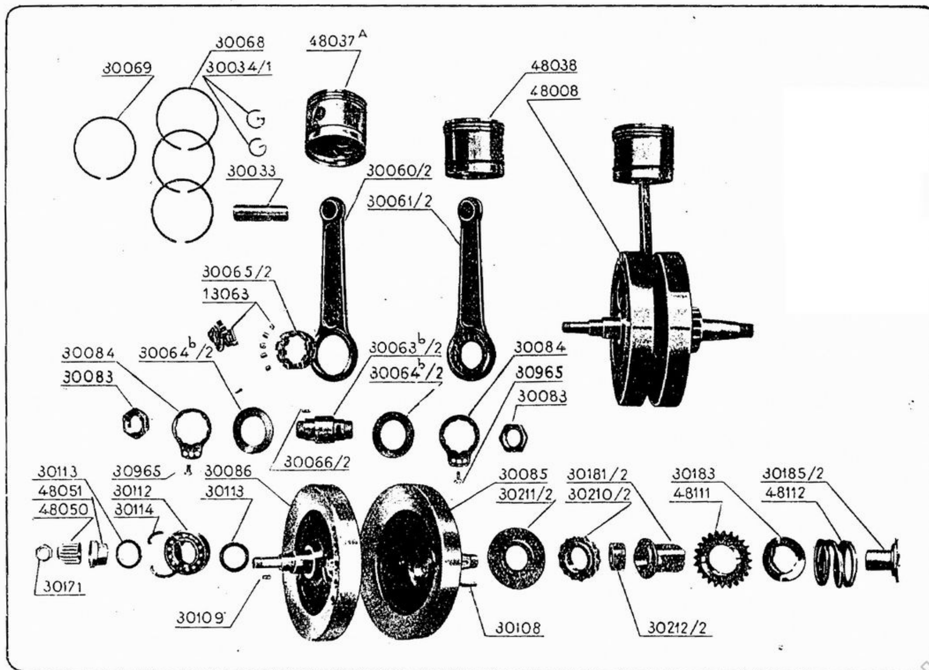
Pistone - biella - volani
