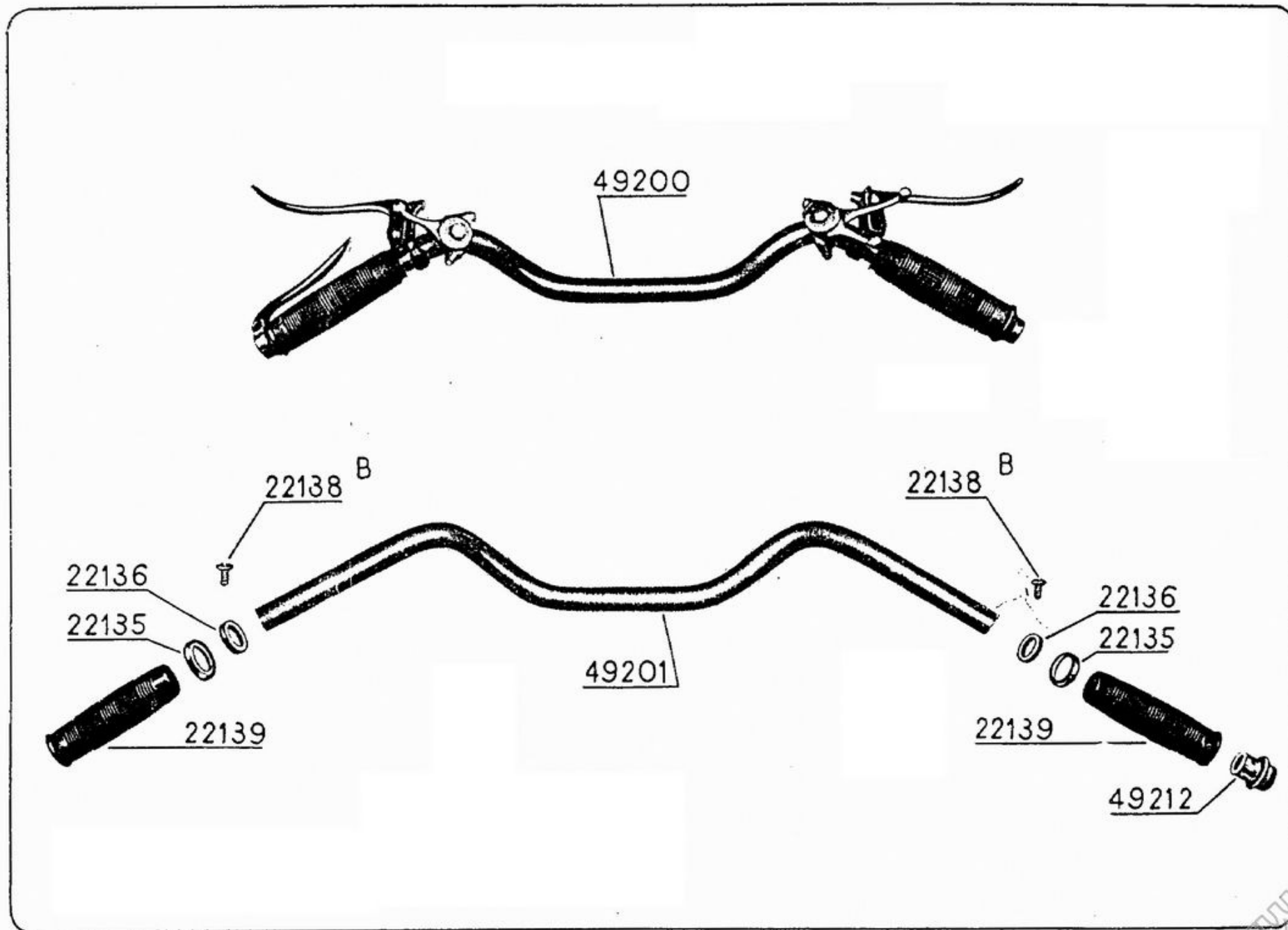
Manubrio
